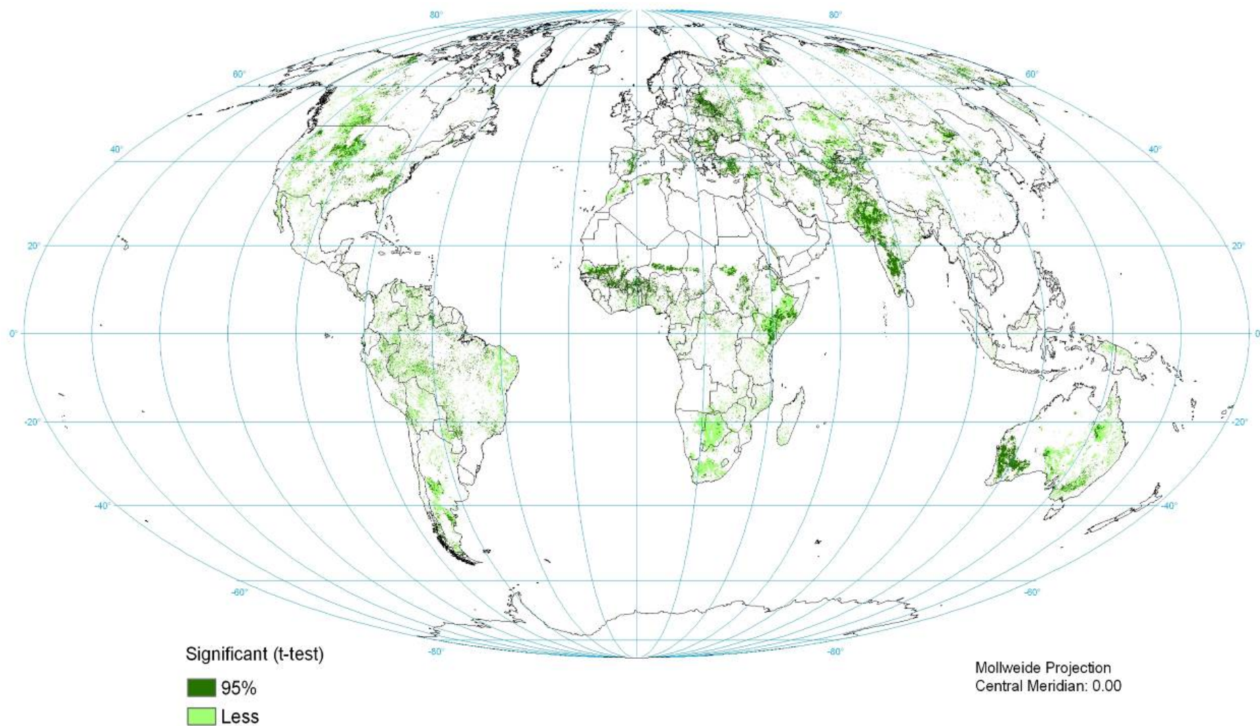
Figure 11. Confidence levels of positive climate-adjusted NDVI, 1981-2003
