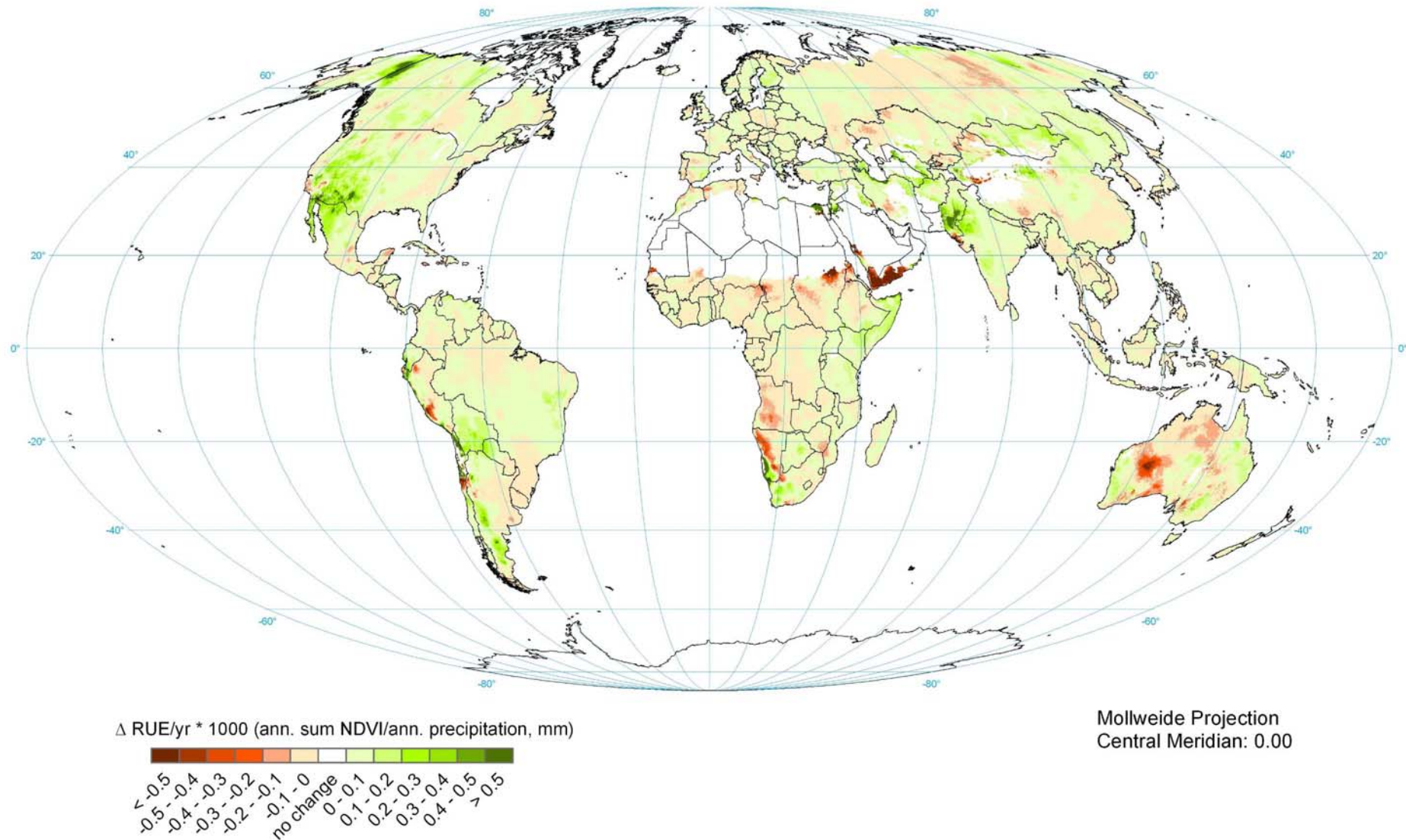
Figure 3. Global change in rain-use efficiency, 1981-2003
