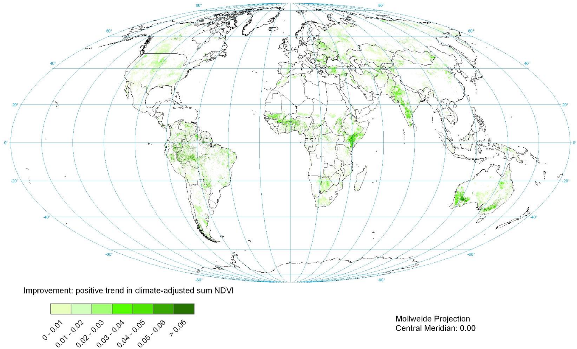
Figure 10. Global trend of positive climate-adjusted NDVI, 1981-2003
