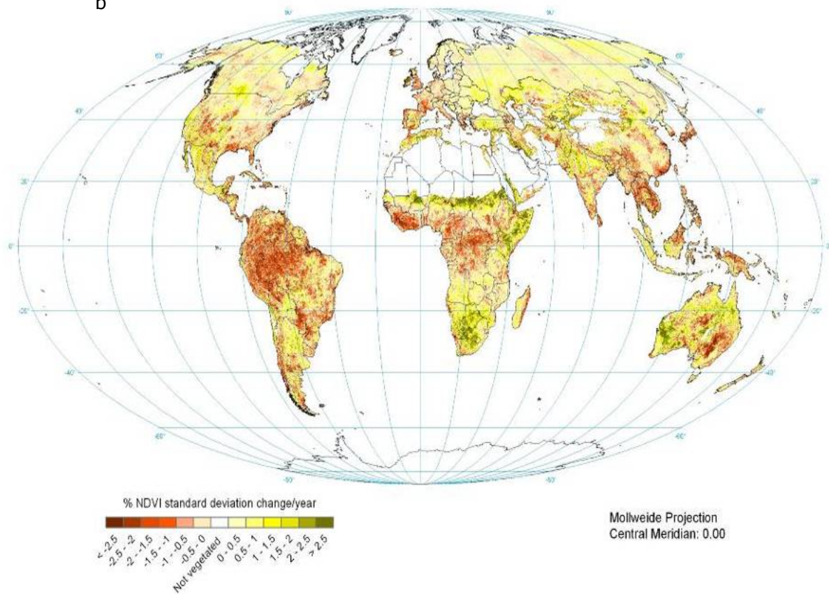
Figure S6. NDVI standard deviation 1981-2003: Pattern (a), trends (b – percentage)
