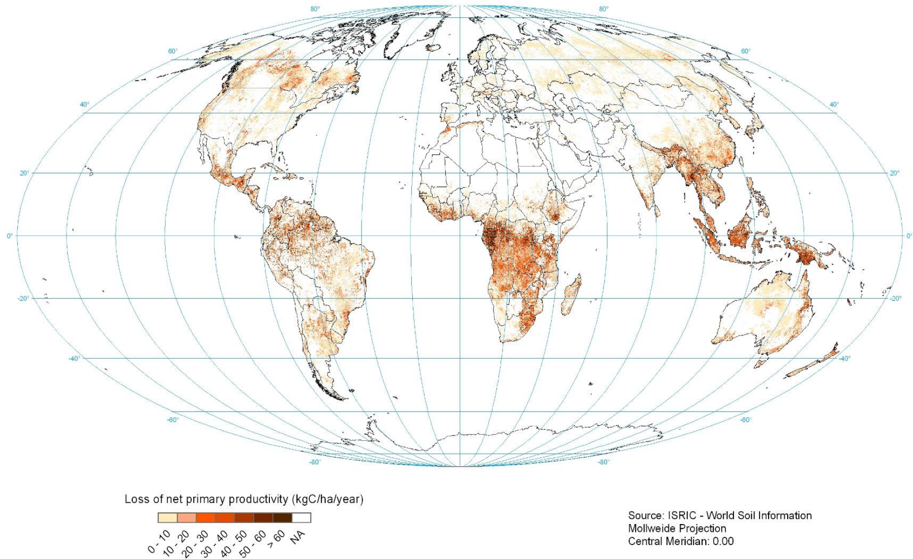
Figure 6. NPP loss in the degrading areas 1981-2003
