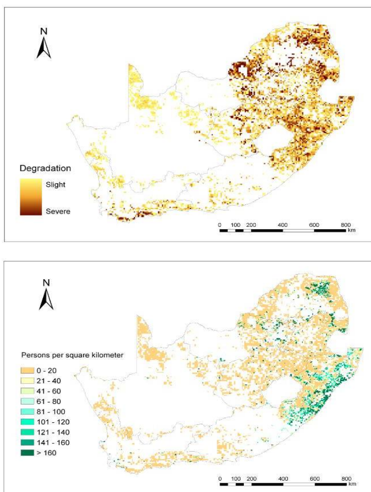
Figure 12. South Africa, land degradation and population affected, 1981-2003
