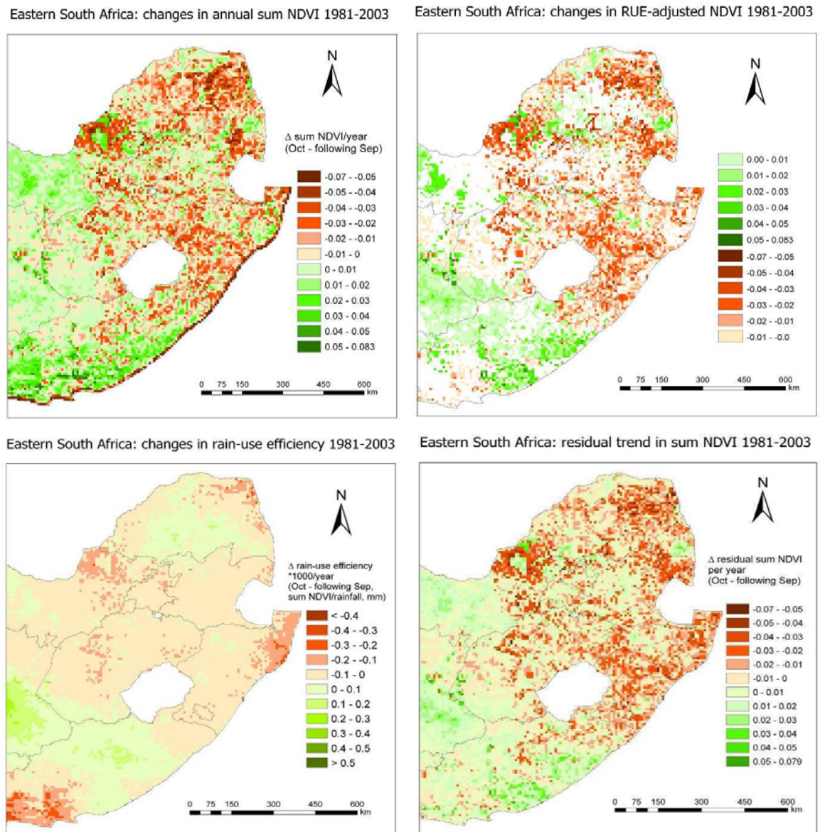
Figure 14. Eastern South Africa: sum NDVI, RUE-adjusted NDVI, rain-use efficiency, and RESTREND
