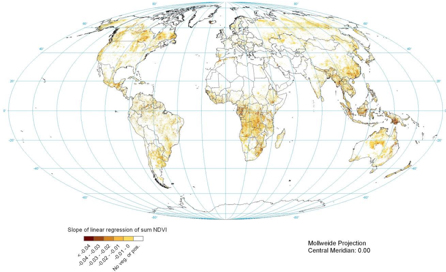
Figure 5. Global negative trend in RUE-adjusted NDVI, 1981-2003
